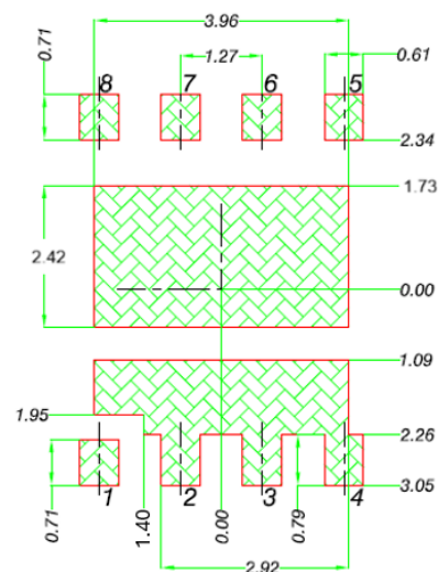
Land Pattern (Only for Reference)
